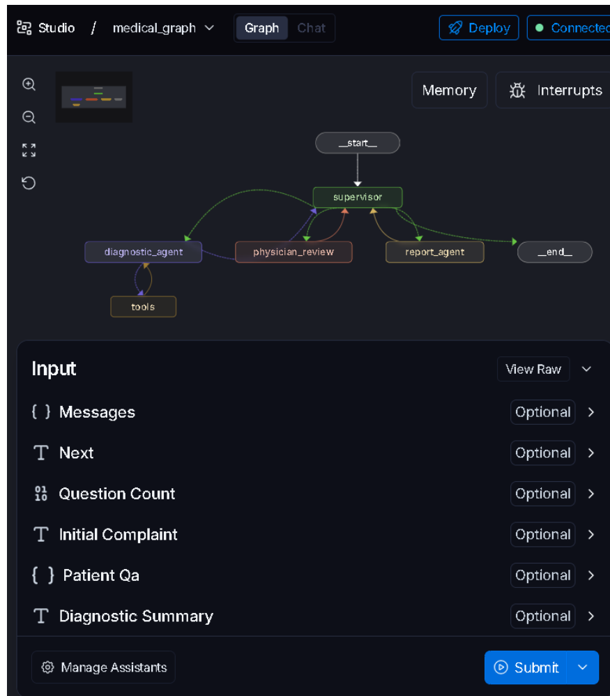
FIGURE 5 – graph langgraph
